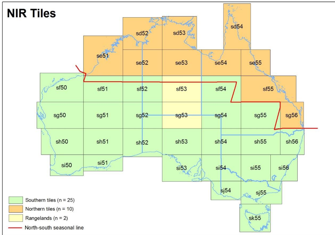
Figure 2: Woody extent data is currently available from 1988-2020 for northern and southern tiles. For rangeland tiles (yellow), data is available from 1989 to 2006.
