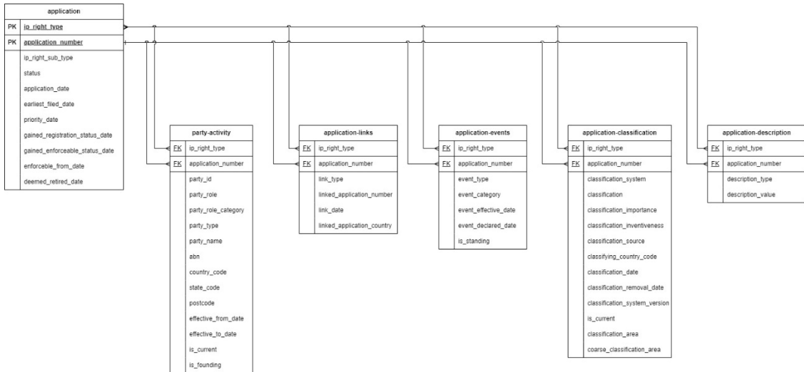
Figure 1: IP RAPID Relational Schema
